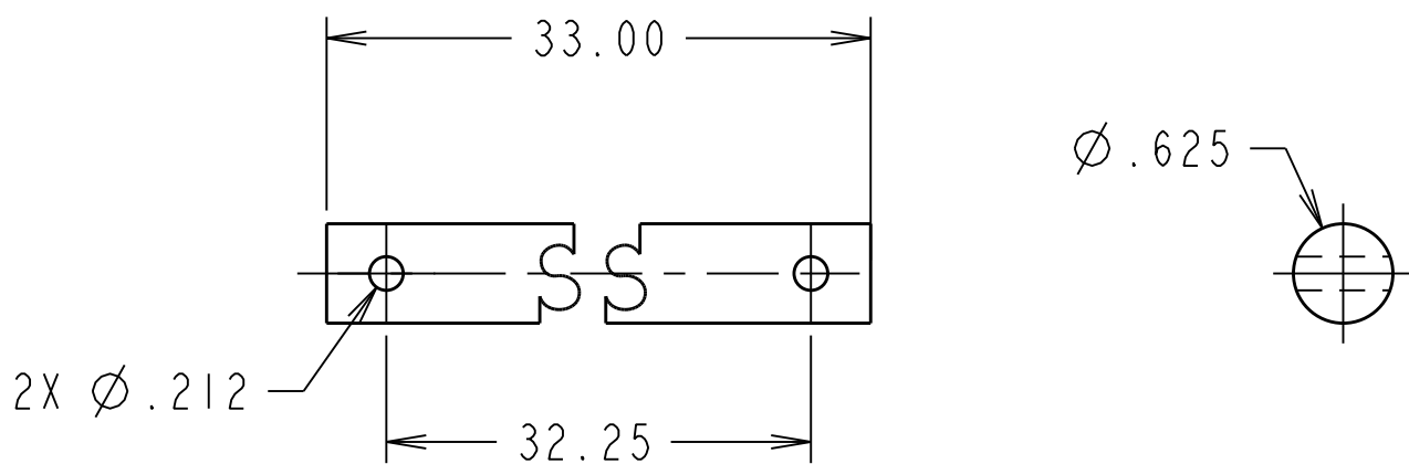
ITEM 24 CDS 1 REQ SCALE 3/4
