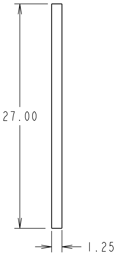
ITEM 3 120-045 2 REQ SCALE 3/20
