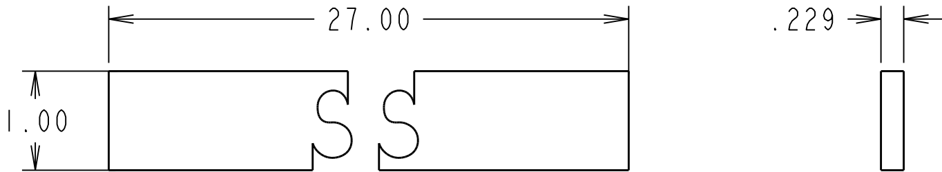
ITEM 28 120-055 1 REQ SCALE 3/4
